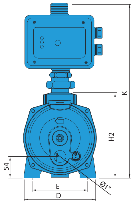
RDW-E WITH PRESSURE CONTROLLER
