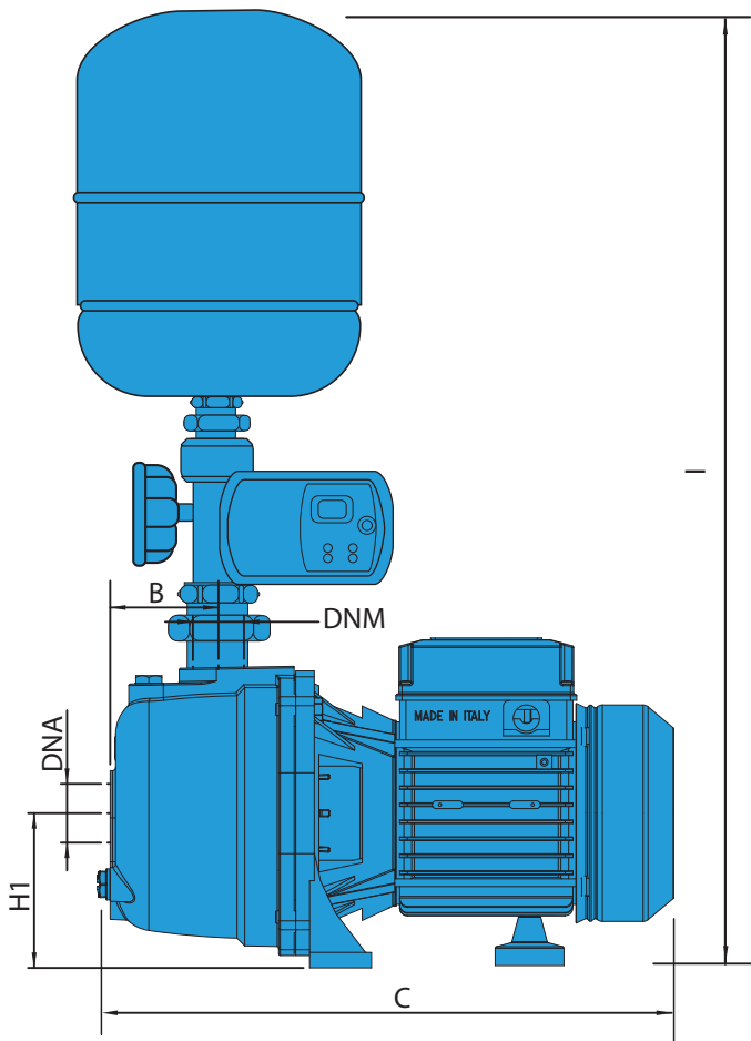
RDW-E WITH PRESSURE SWITCH
