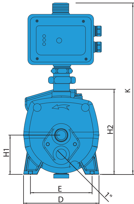
RDW-E WITH PRESSURE CONTROLLER
