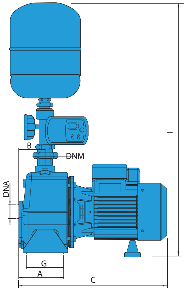
RDW-E WITH PRESSURE SWITCH
